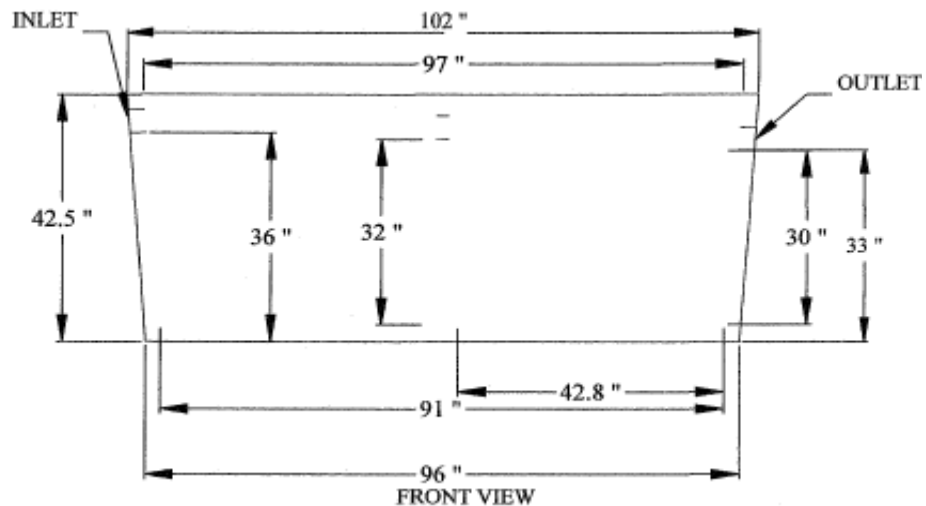
FRONT VIEW
